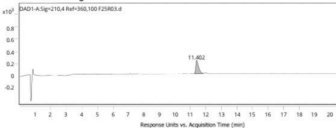
UV chromatogram
